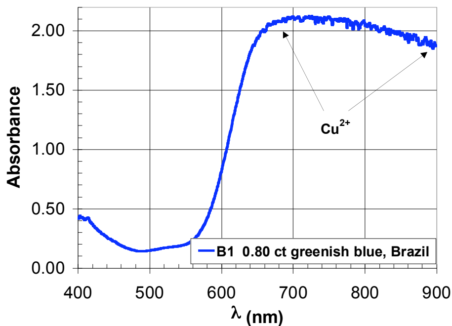
Elbaite Tourmaline, StellarNet EPP2000
