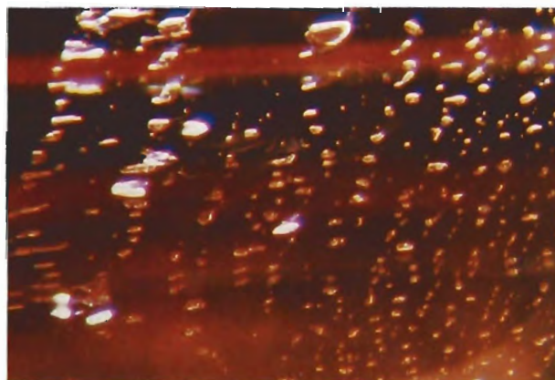
Figure 13. These parallel rows of two-phase inclusions are a diagnostic internal feature of topaz. Magnified 16×.
